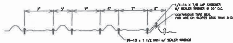
FASTENER PATTERN TYPE 2 AND AT EAVE & VALLEY
